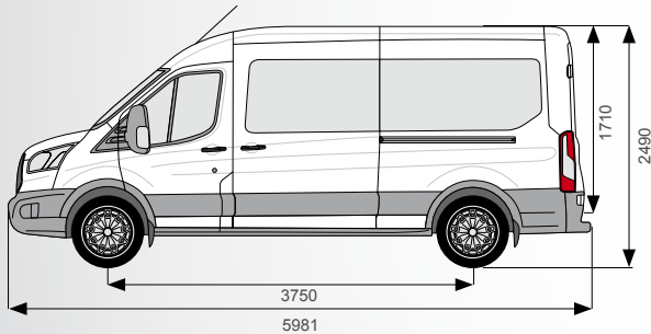
FORD TRANSIT L3 H2
